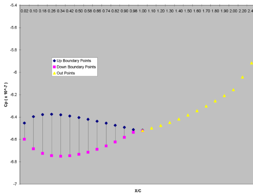
Fig. 4 Pressure distribution around the aircraft of Fig.3, for constant source distribution and speed 1 Mach.
