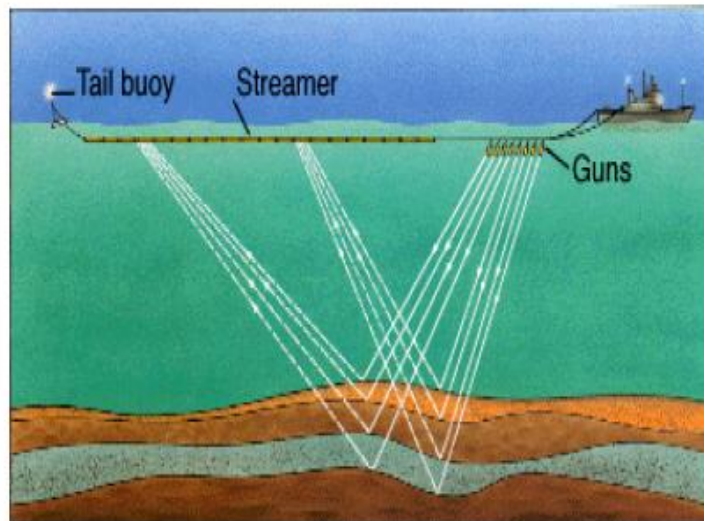
Fig. 2 Non-linear Real-time Expert Seismology.
