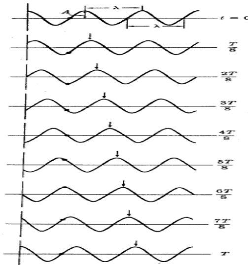
Fig. 5 A sinusoidal transverse wave traveling toward the right, at intervals 1/8 of a period.
