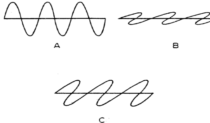
Fig. 7 Transverse waves, traveling in the same direction, but lying in different planes from one another.
