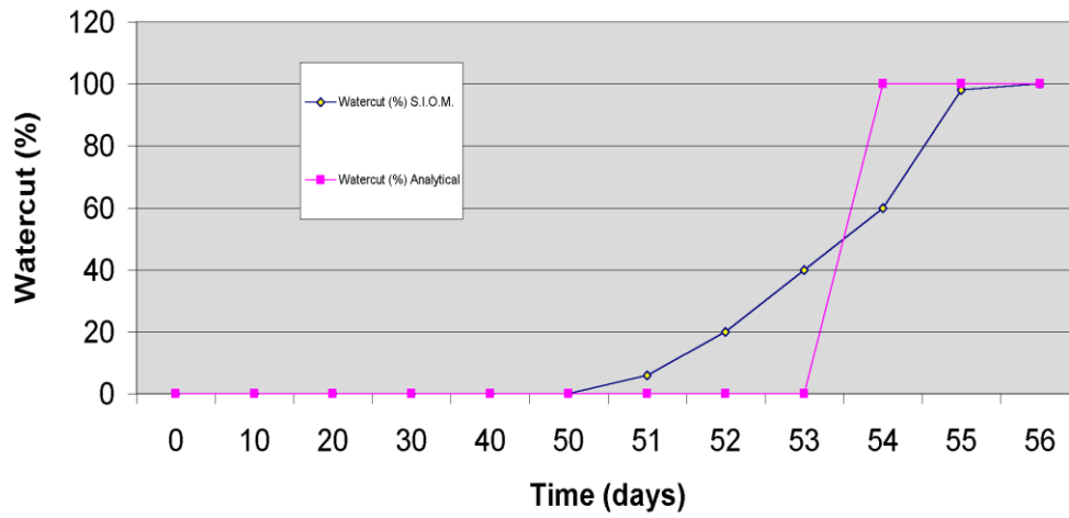
Fig. 1 Multiphase Flow of Oil Reservoir Mixed with Water.
