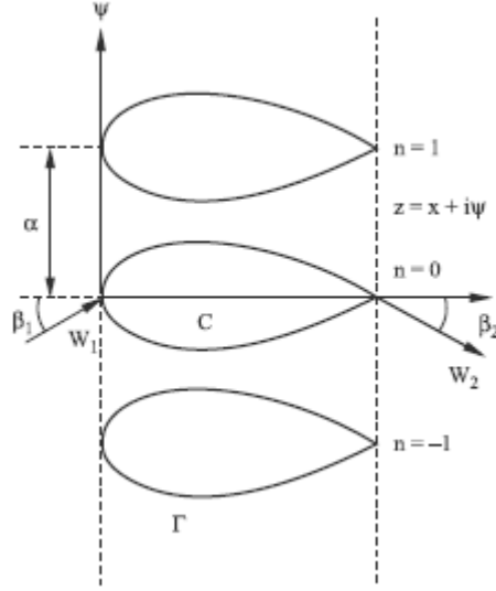
Fig. 2 A lattice of airfoils in an axial turbine
